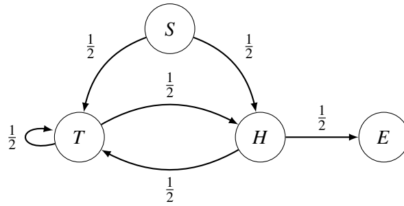
Figure 5: Flipping a fair coin until two heads in row.
